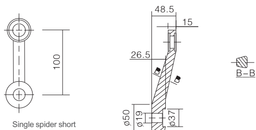
Single spider short
