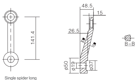
Single spider long
